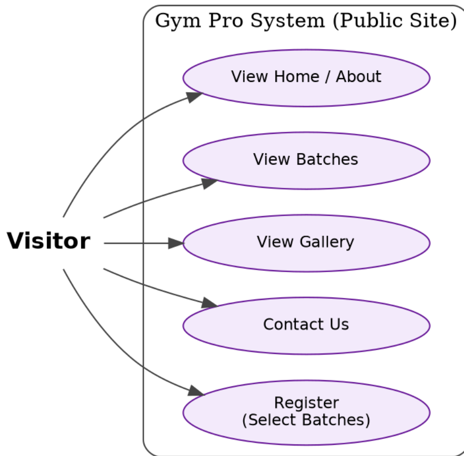
Fig 4.1(a): Use-case diagram – Visitor
