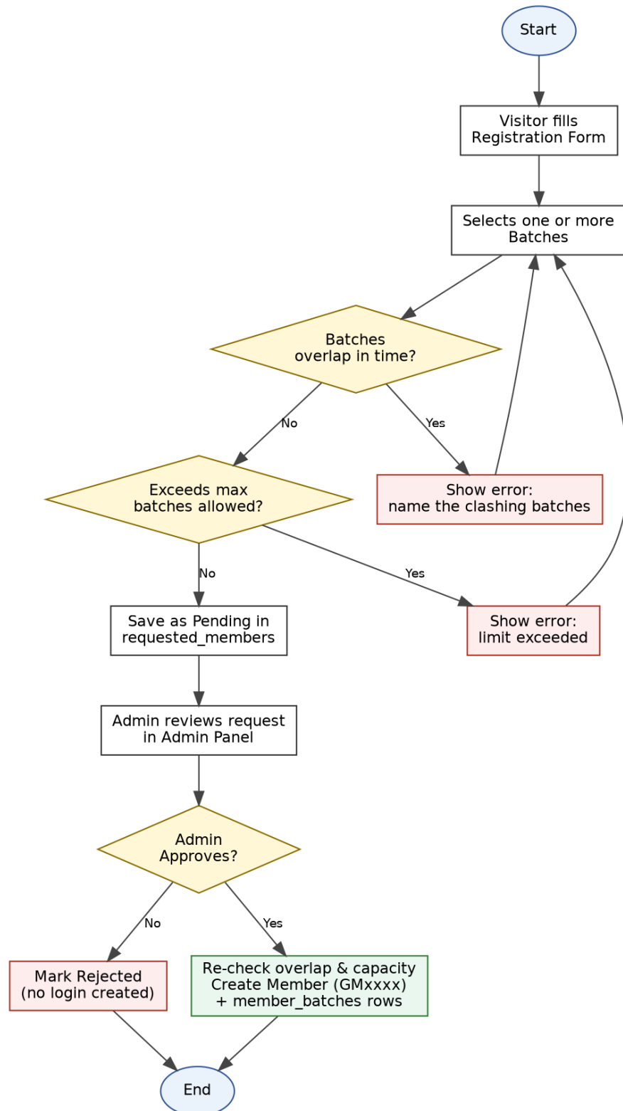
Fig 4.5: Flowchart of the Registration & Approval process
